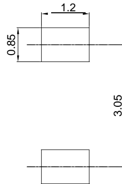
SOD-123
