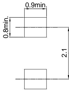
SOD-323
