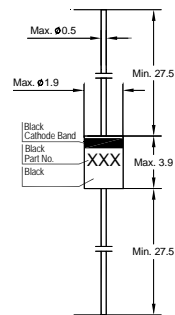
Glass Case DO-35 Dimensions in mm
